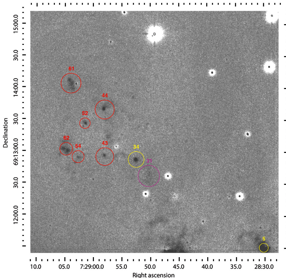
Fig. 4. [S II]-continuum subtracted image of NGC 2366 - FOV2, taken from NAO Rozhen. Properties of marked objects are given in Table 2.
